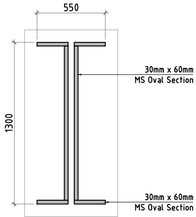
- TOP PLAN @ 750MM LVL.
