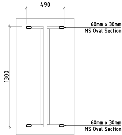
- PLAN @ 300MM LVL.
