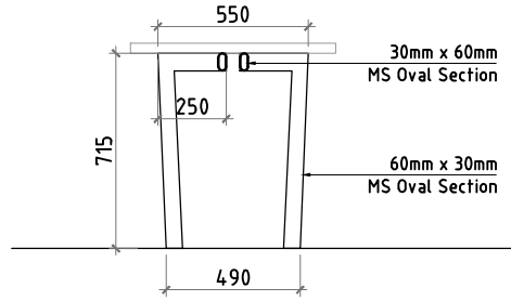
- FRONT SECTIONAL ELEVATION
